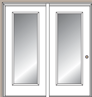
**Patio Unit (Hinged off the Mull Post) R-H Active / L-H Swing
